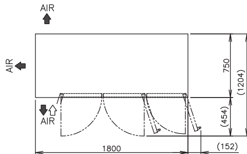
VIEW A(1/10)
